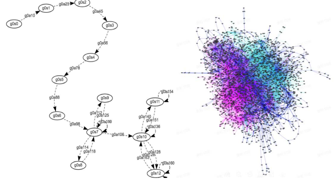
Figure 2: DAG Model
